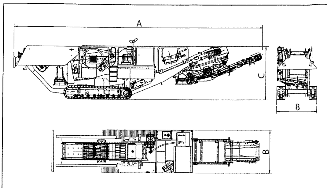
Abbildung 3-3 LT96S in Transportposition
